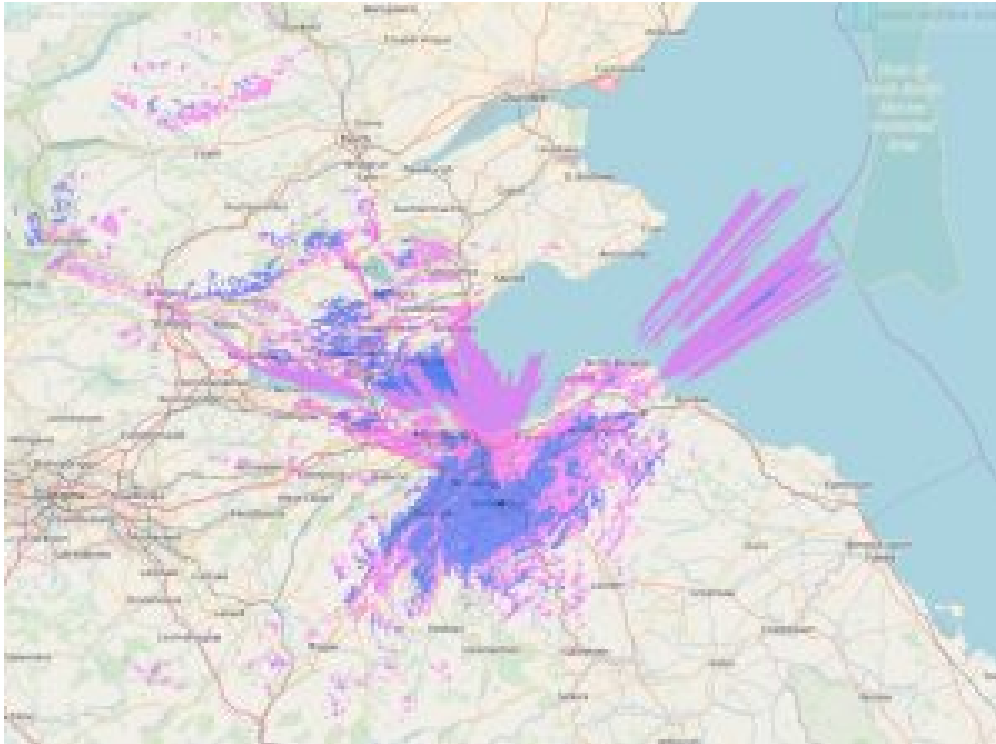
GB7SQ Dalkeith DMR Predicted Coverage
